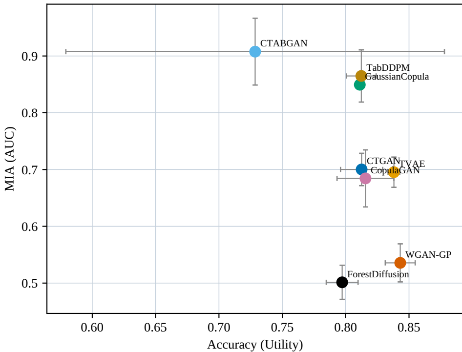
CDC Diabetes: Accuracy (Utility) vs MIA (AUC)
